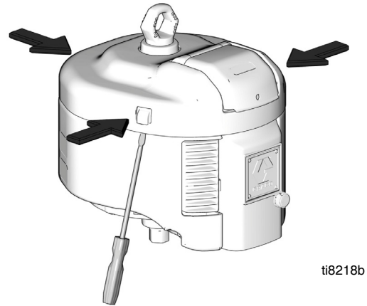
FIG. 2: Remove Air Motor Cover
