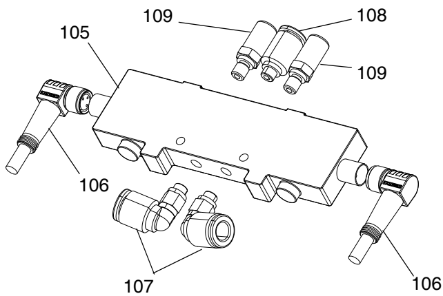
FIG. 9: Assemble Fittings
