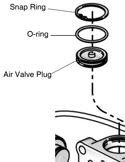
FIG. 11: Remove Existing Air Valve Plug
