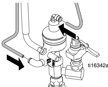
Double-Acting Gun
