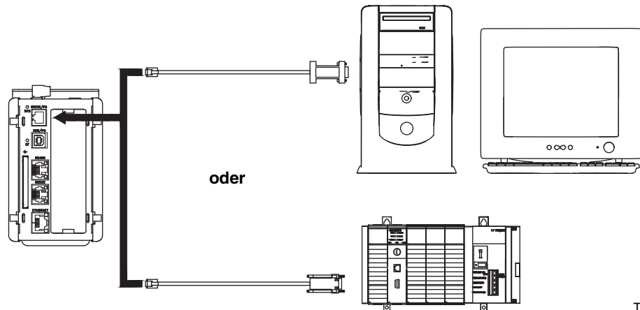
ABB. 7: RS232/PG-Kommunikationsanschlüsse
