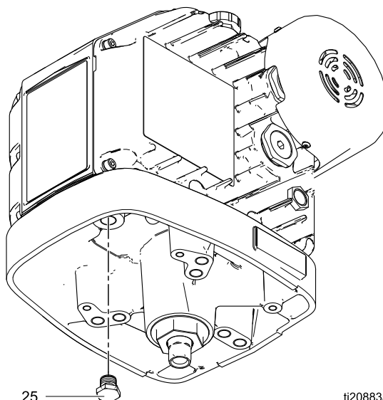
Figure 14 Olieaftapplug
