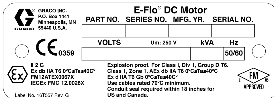
Figure 1 Identificatielabel basismotor
