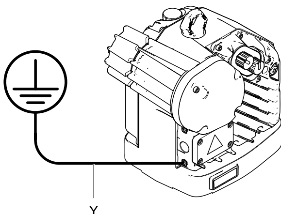
Figure 8 Massadraad
