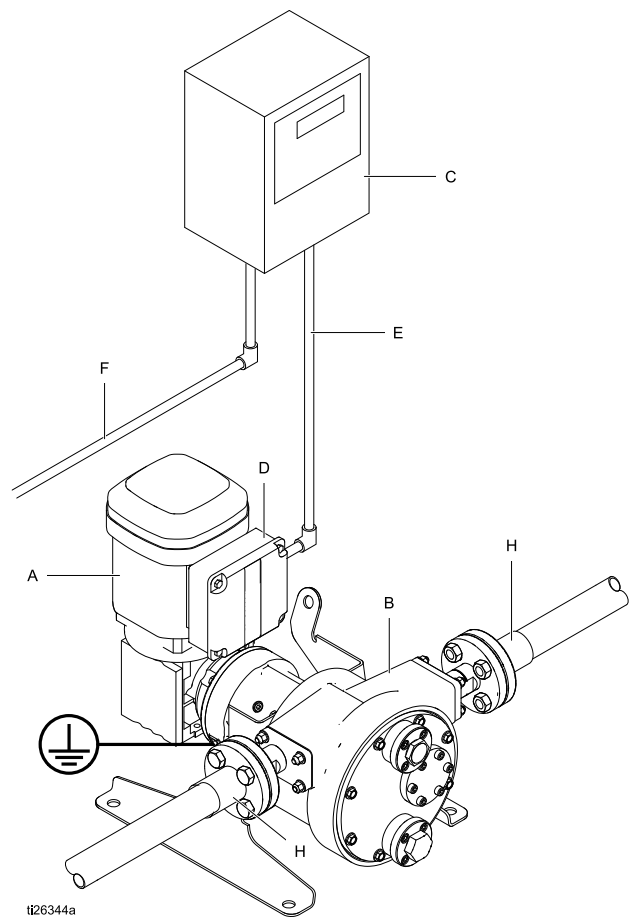
AC-pomp met VFD
