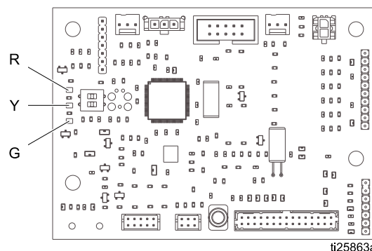
Figure 16 Schakelbord
