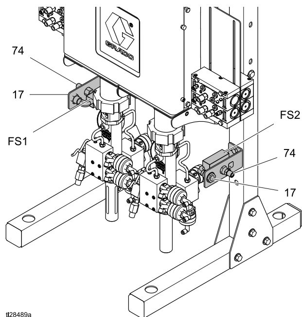
Figure 16 溶剂连接
