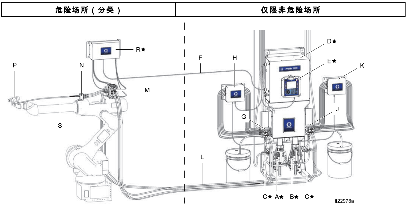
Figure 10 典型安装
