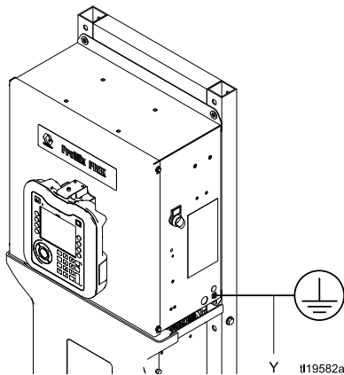
Figure 20 接地螺丝及电源开关
