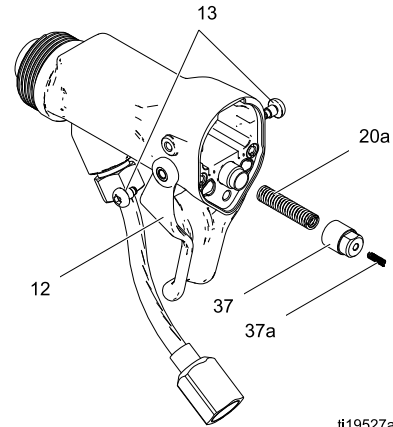
Figure 29 卸下帽子和弹簧
