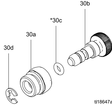
Figure 37 扇形空气调节阀
