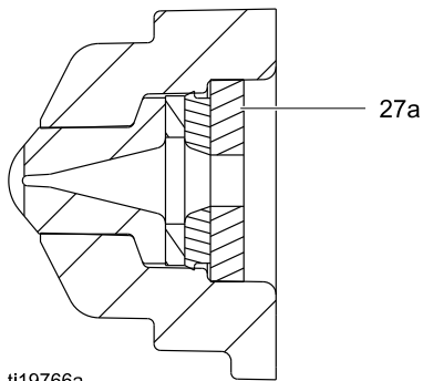
Figure 22 喷嘴垫片
