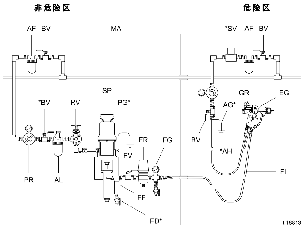
Figure 10 典型安装
