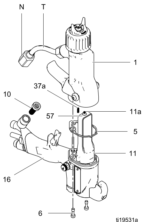
Figure 28 枪筒安装
