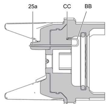
Figure 24 更换电极
