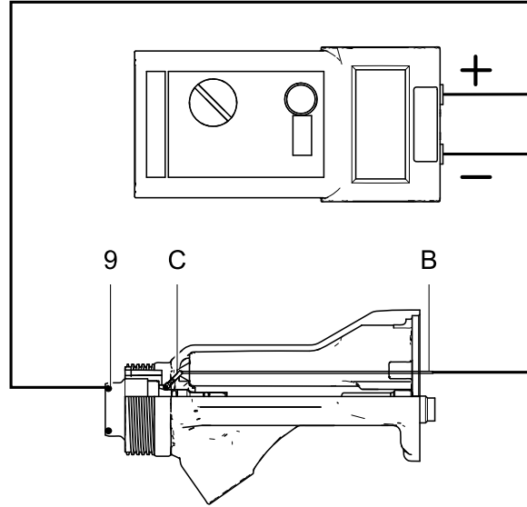
Figure 19 测试枪筒电阻
