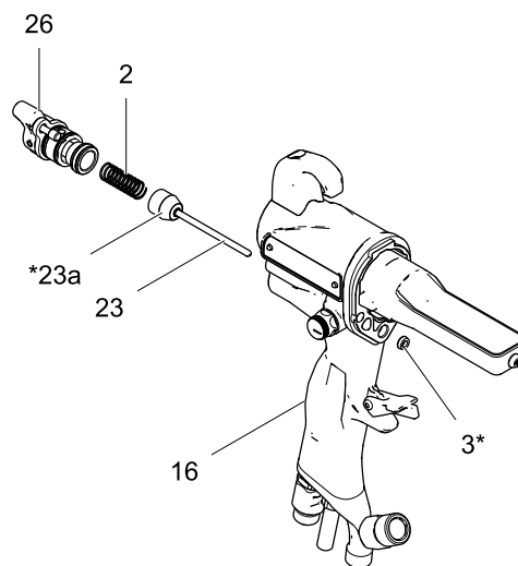
Figure 41 空气阀
