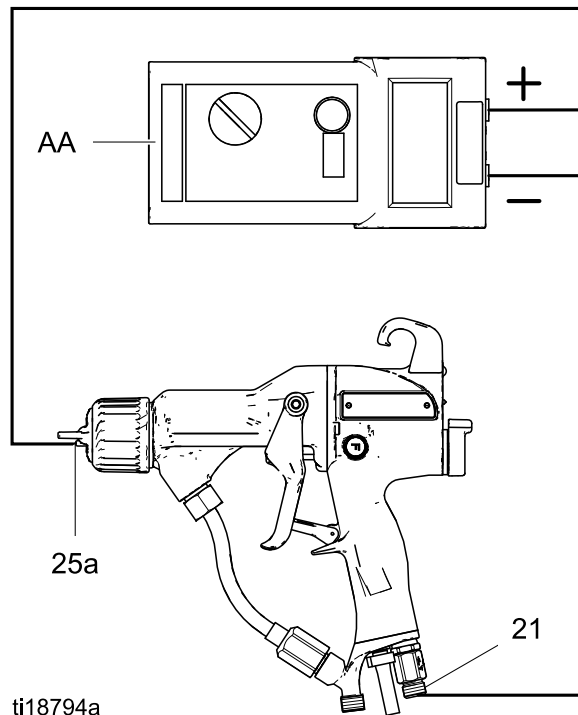
ti18794a Figure 17 测试喷枪的电阻
