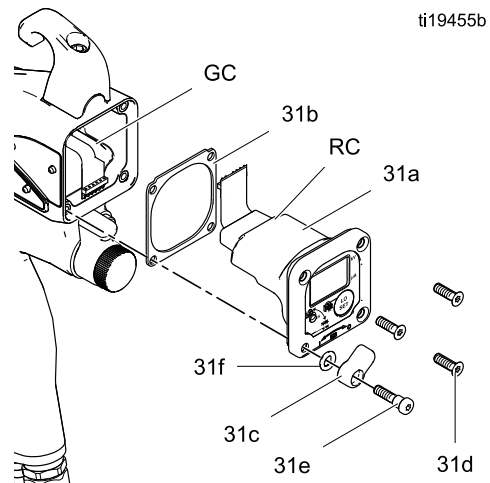
Figure 42 智能模块
