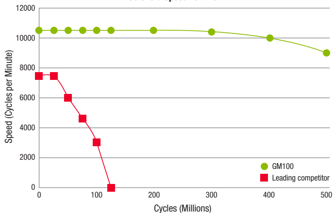
Solenoid Speed vs. Life
