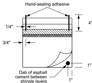
Figure 14-22: Hand seal caps as shown.
