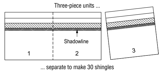
Figure 14-19: Separate to make 3 cap shingles.
