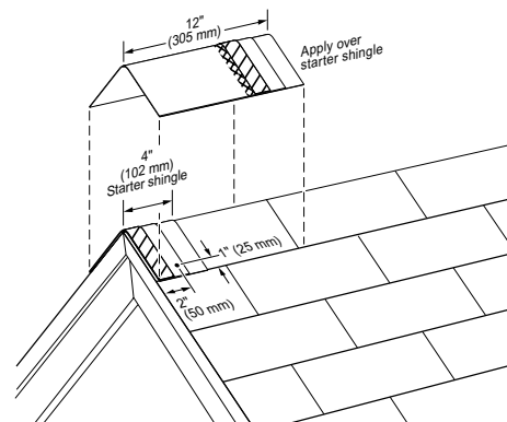
Figure 14-20: Apply a full cap shingle over the starter shingle.
