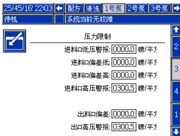
Figure 47 泵屏幕 3，已启用压力监控
