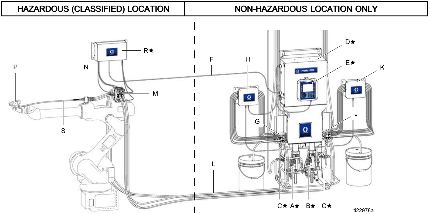
Figure 10 Typical Installation
