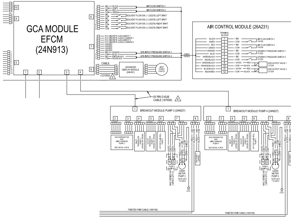
Figure 33 Electrical Schematic, Sheet 2, Part 2
