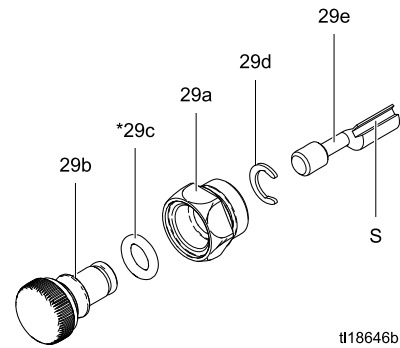
Figure 33 雾化空气限流阀
