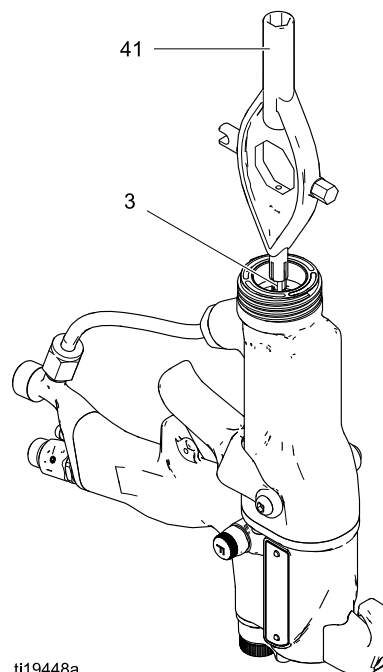
Figure 21 电极更换
