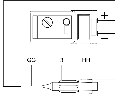
Figure 19 测试电极电阻
