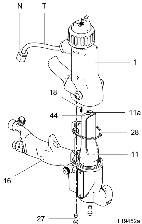
Figure 25 枪筒安装
