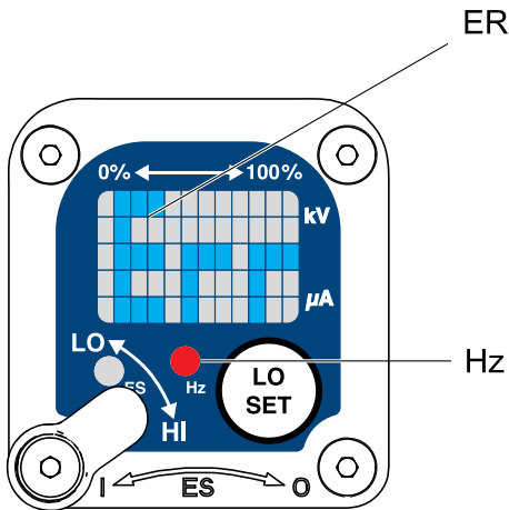
ti19338a Figure 3 错误显示窗
