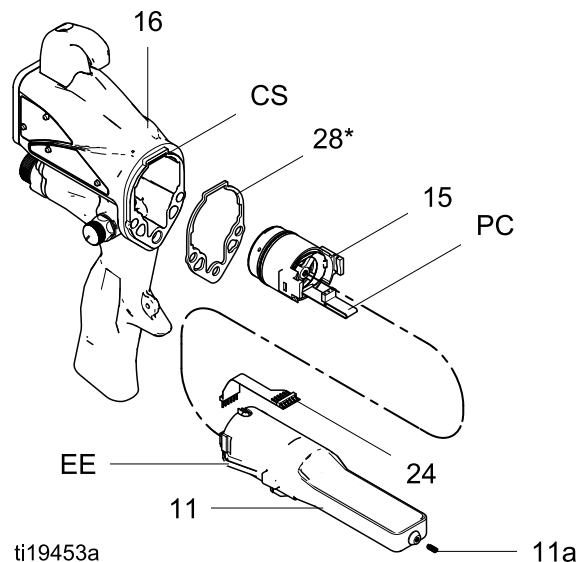
Figure 27 供电电源
