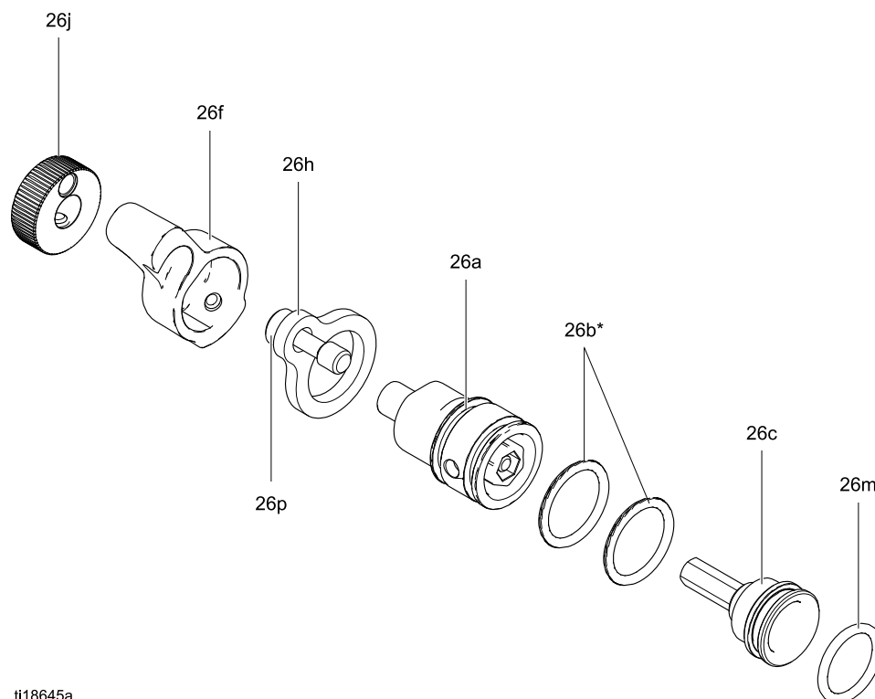
Figure 35 ES On-Off 和流体调节阀
