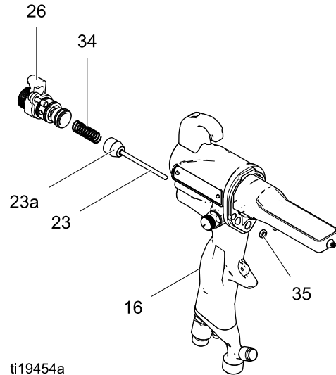
Figure 37 空气阀
