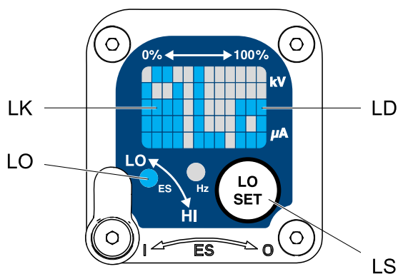
Figure 9 低压锁定屏幕
