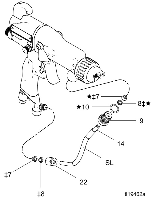
Figure 31 流体管
