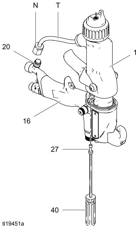
Figure 24 枪筒拆卸
