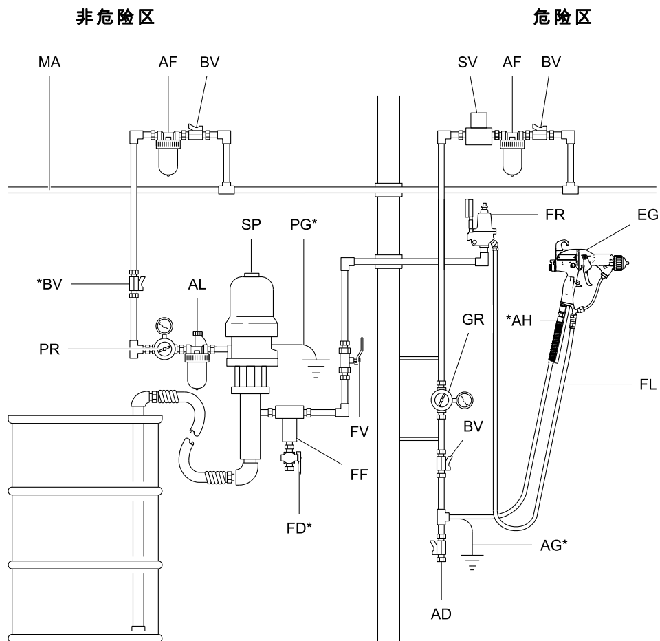
Figure 10 典型安装
