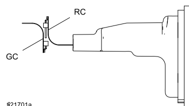
Figure 39 对齐带状电缆
