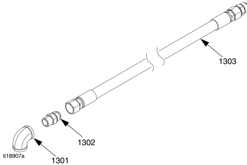
FIG. 24: Inlet Hose Assembly Kits
