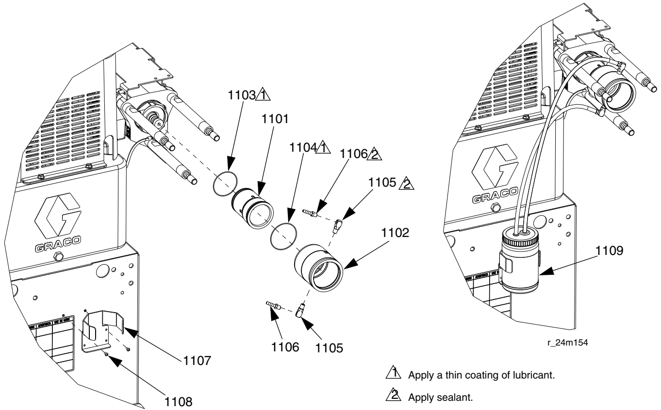
FIG. 25: Lubrication Kit
