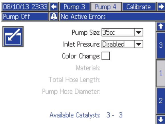
Figure 17 Fourth (Catalyst) Pump Screen
