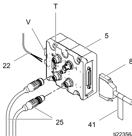
Figure 25 Pump Control Module Connections
