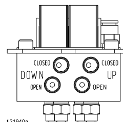
Figure 21 Tubing Connections at Solenoid Manifold, to Pump Outlet Manifold
