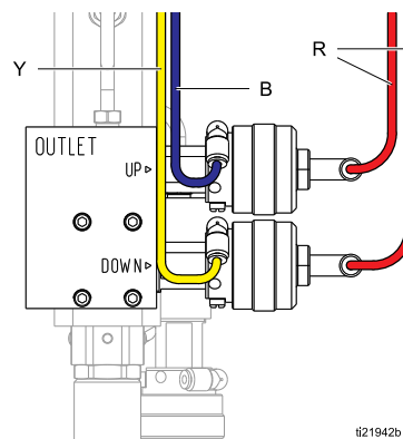
Figure 22 Outlet Manifold Tubing Connections
