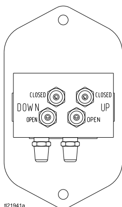
Figure 19 Tubing Connections at Solenoid Manifold, to Pump Inlet Manifold
