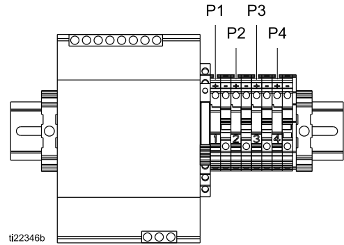
Figure 11 48 VDC Power Supply Connection Points
