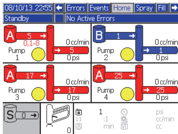
Figure 18 PD2K Home Screen (Advanced Display Module)
